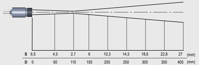
CT 1ML/2ML CF, D:S = 40:1 (champ éloigné = 12:1)
