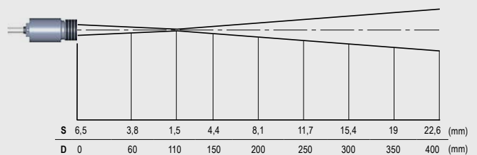
CT 1MH/1MH1/2MH/2MH1 CF, D:S = 75:1 (champ éloigné = 14:1)
